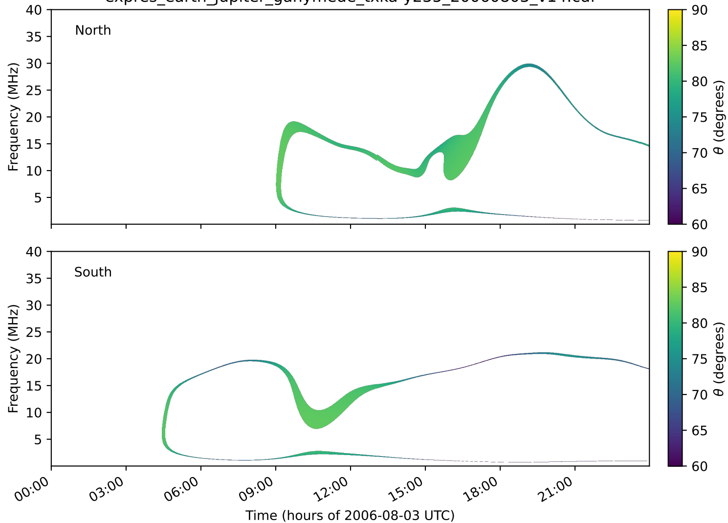
expres_earth_jupiter_ganymede_txka-y235_20060803_v14.cdf
