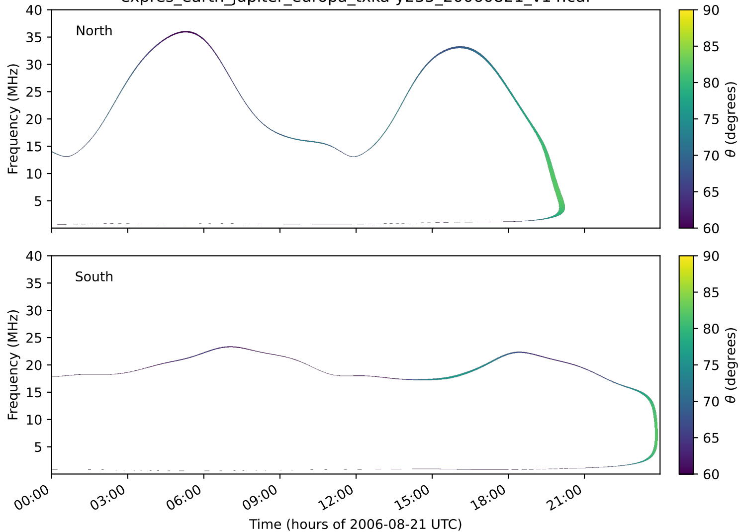
expres_earth_jupiter_europa_txka-y235_20060821_v14.cdf
