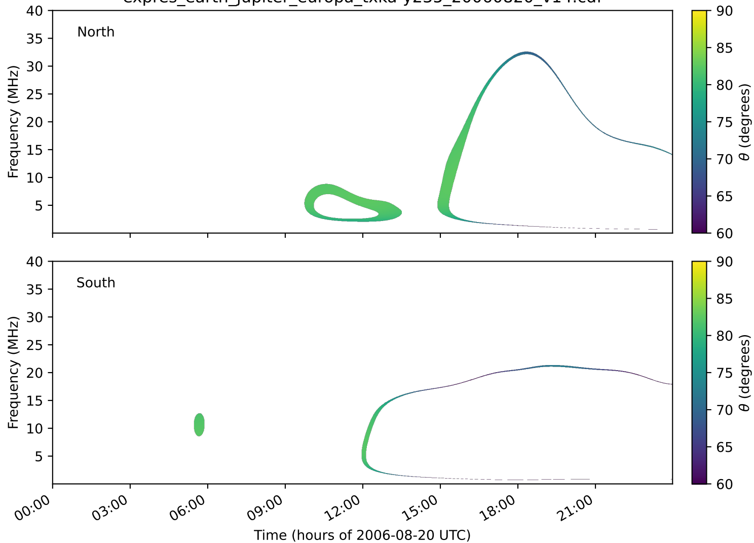
expres_earth_jupiter_europa_txka-y235_20060820_v14.cdf
