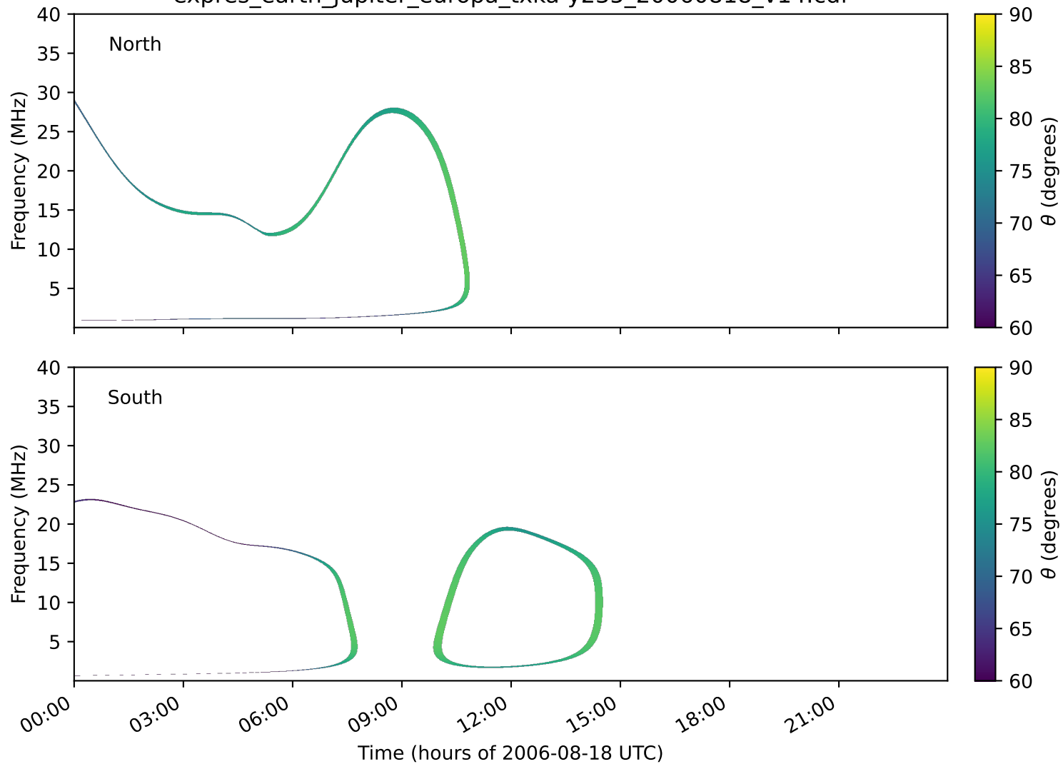
expres_earth_jupiter_europa_txka-y235_20060818_v14.cdf
