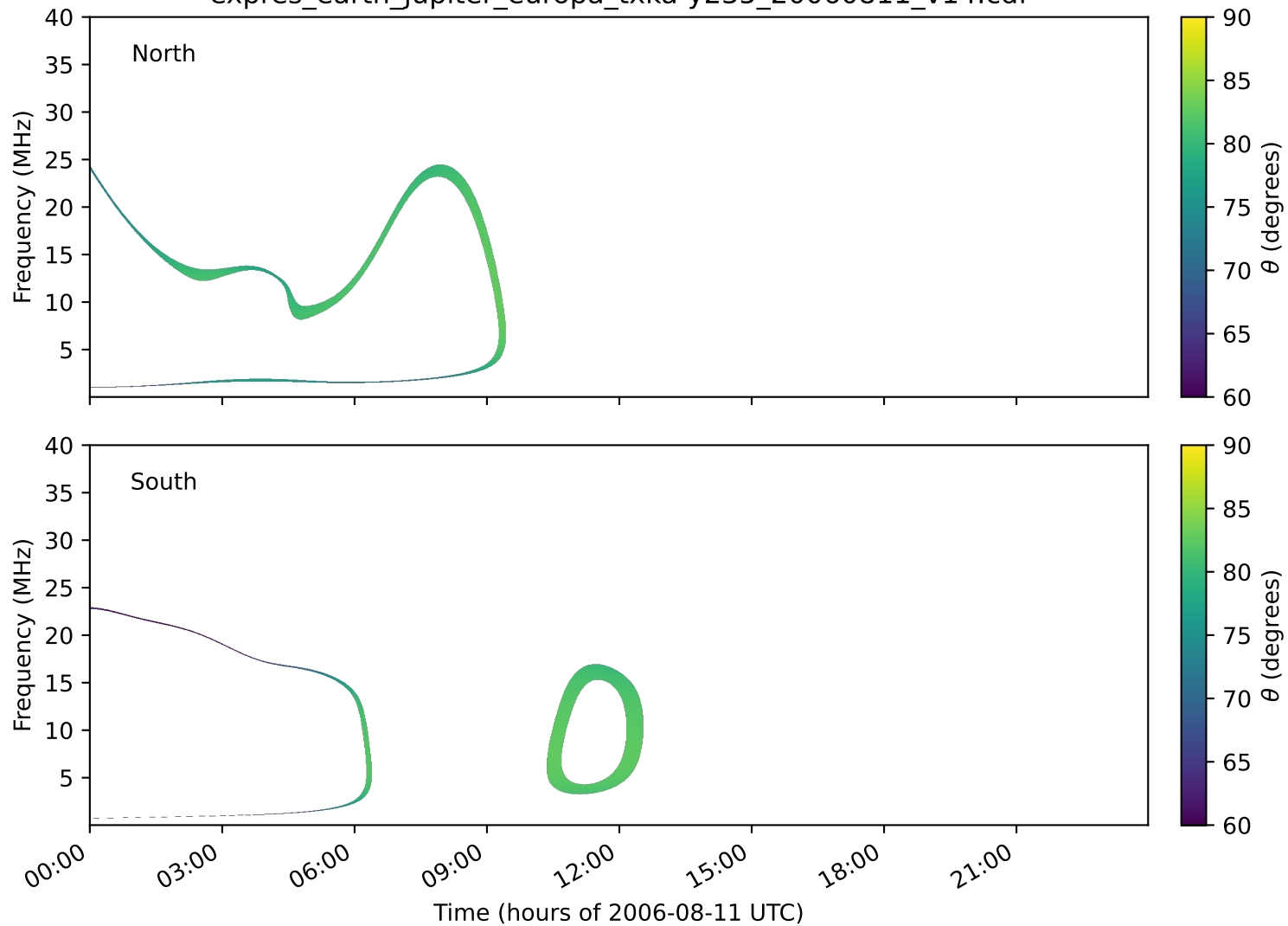
expres_earth_jupiter_europa_txka-y235_20060811_v14.cdf
