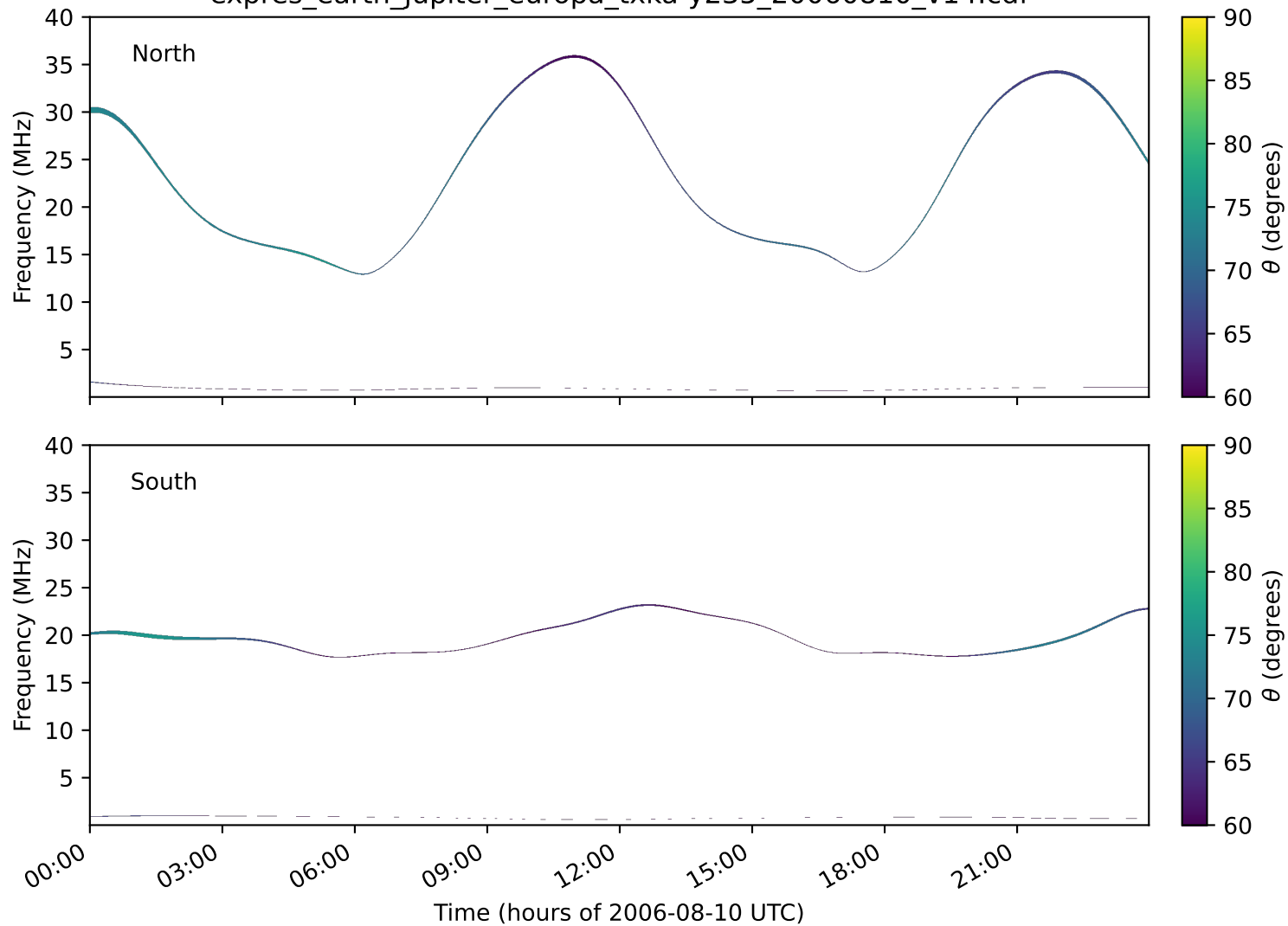
expres_earth_jupiter_europa_txka-y235_20060810_v14.cdf
