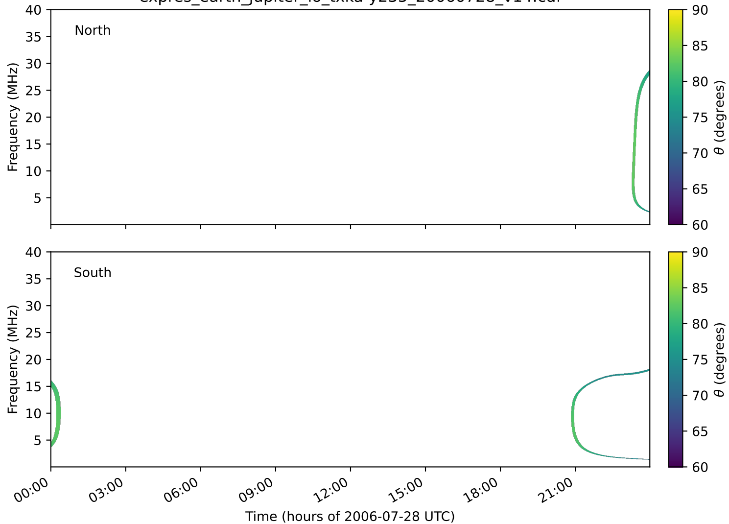
expres_earth_jupiter_io_txka-y235_20060728_v14.cdf
