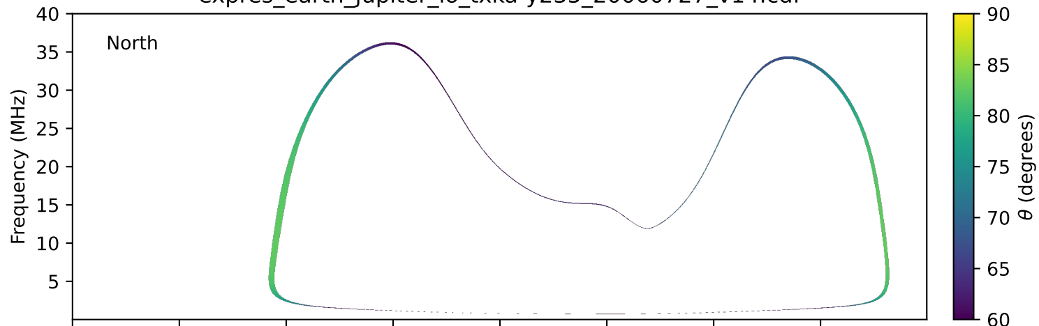
expres_earth_jupiter_io_txka-y235_20060727_v14.cdf
