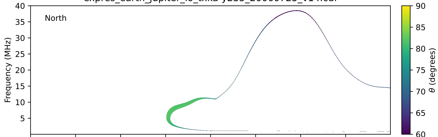
expres_earth_jupiter_io_txka-y235_20060725_v14.cdf
