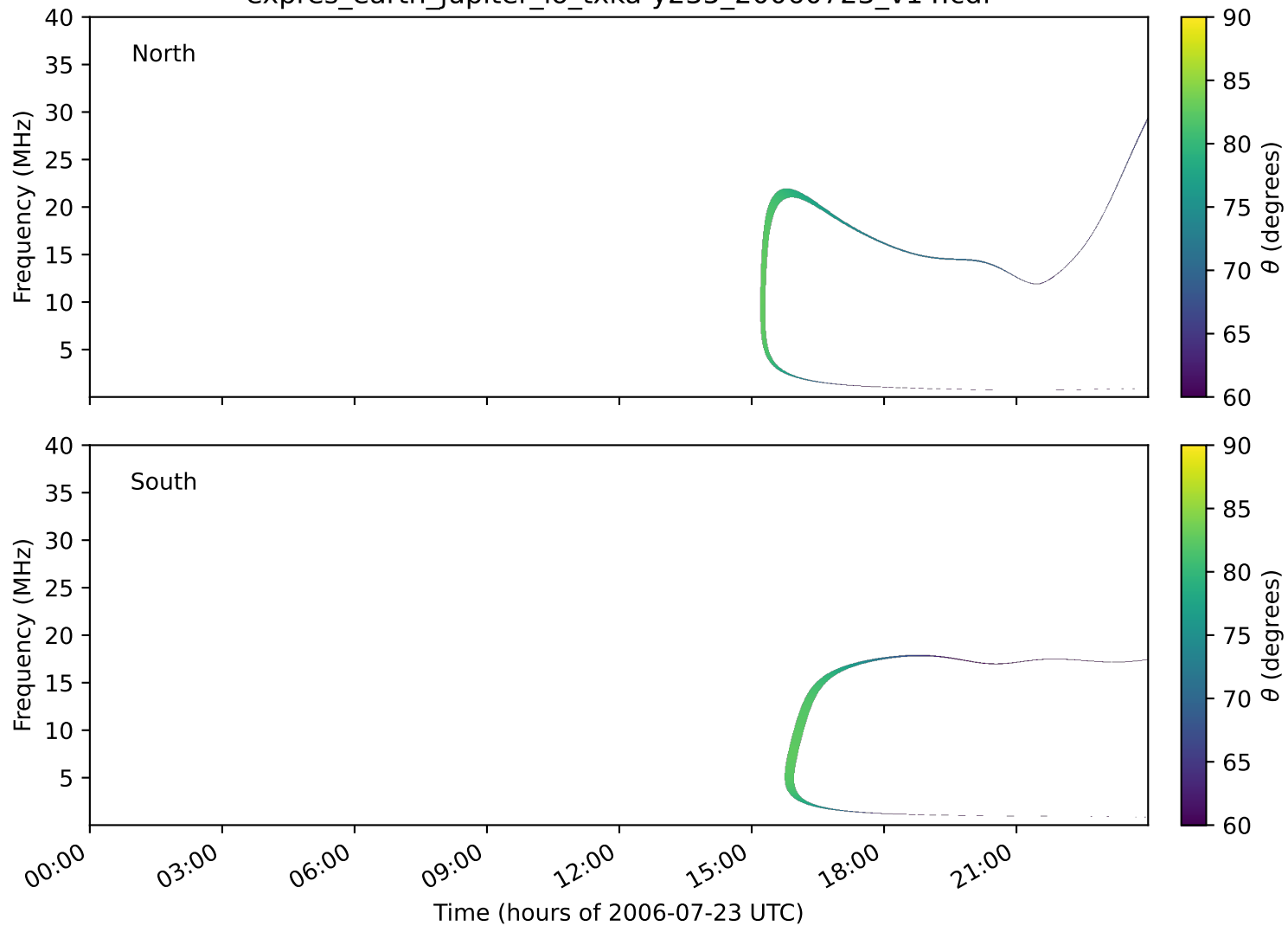
expres_earth_jupiter_io_txka-y235_20060723_v14.cdf
