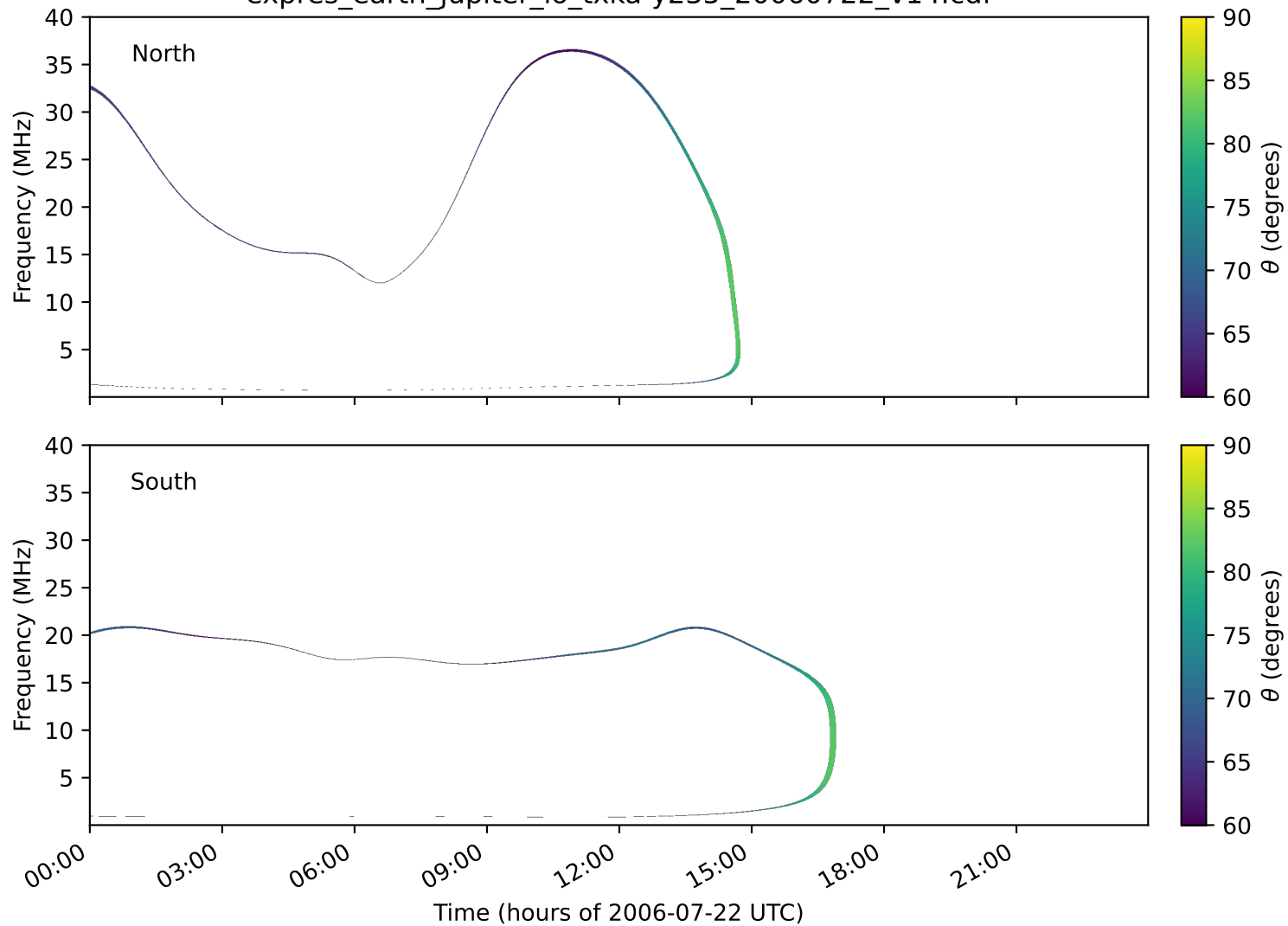
expres_earth_jupiter_io_txka-y235_20060722_v14.cdf
