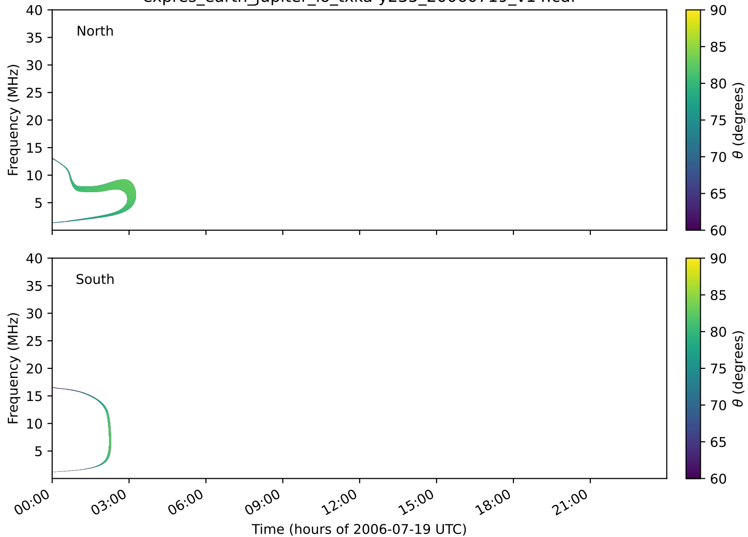
expres_earth_jupiter_io_txka-y235_20060719_v14.cdf
