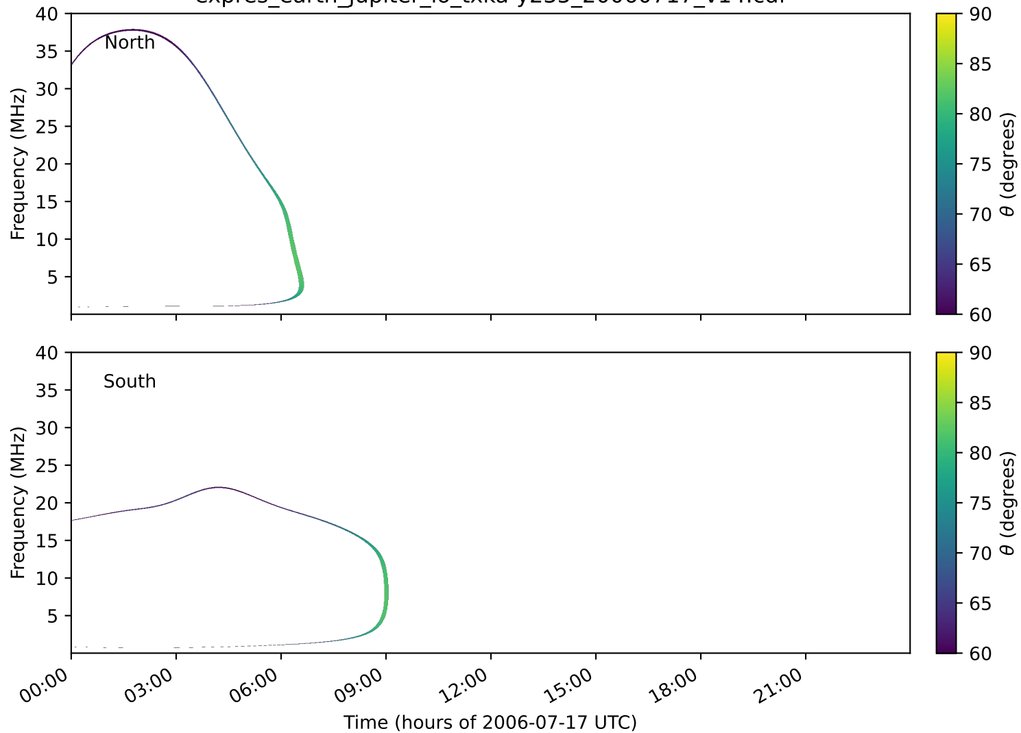
expres_earth_jupiter_io_txka-y235_20060717_v14.cdf
