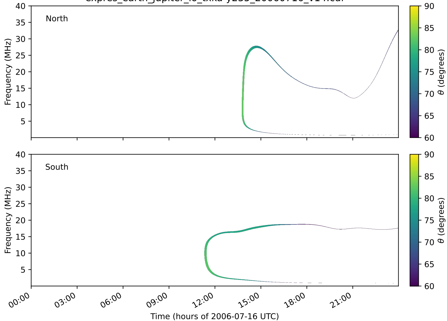
expres_earth_jupiter_io_txka-y235_20060716_v14.cdf
