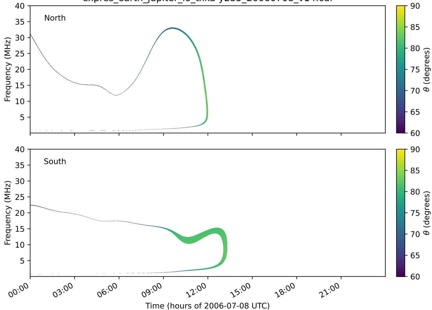
expres_earth_jupiter_io_txka-y235_20060708_v14.cdf
