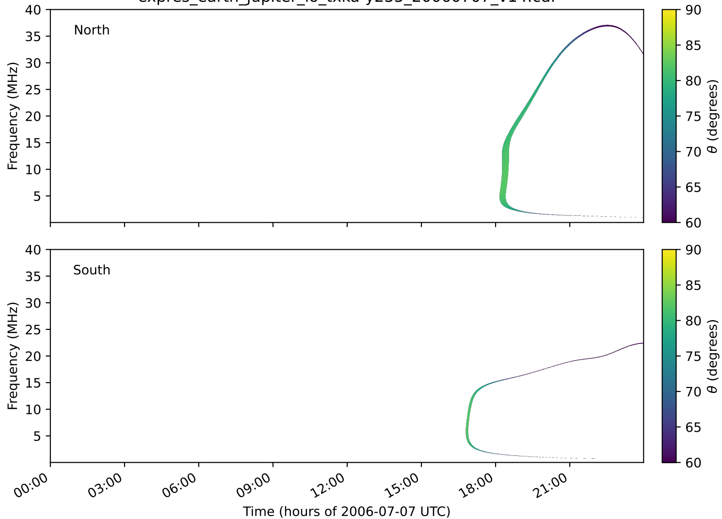
expres_earth_jupiter_io_txka-y235_20060707_v14.cdf
