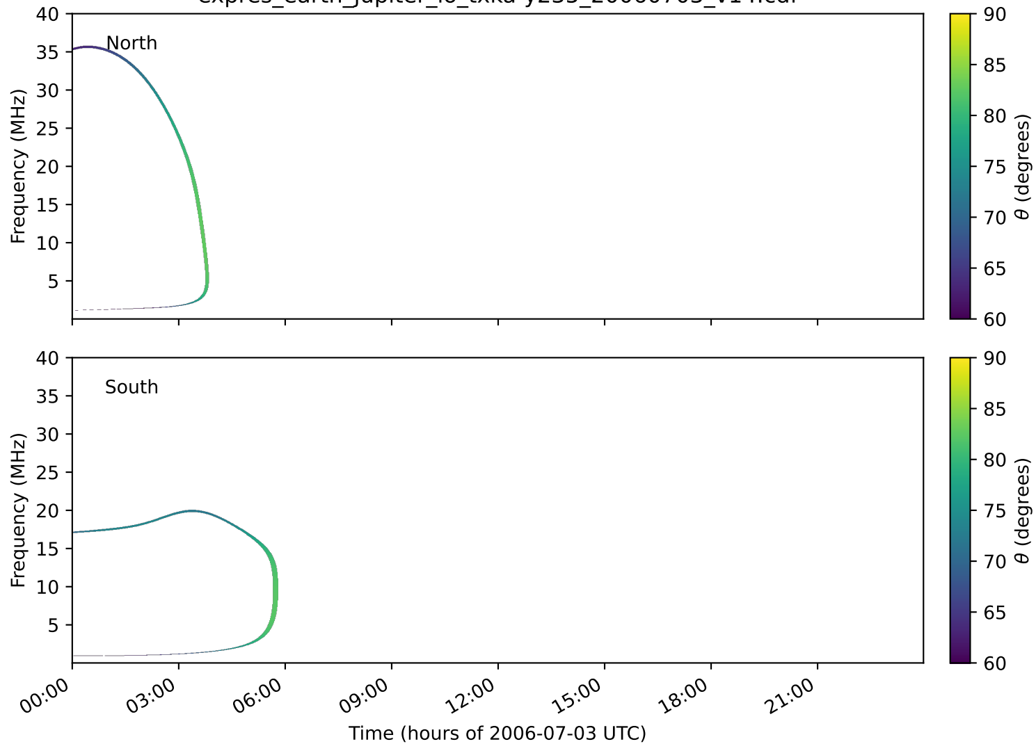
expres_earth_jupiter_io_txka-y235_20060703_v14.cdf
