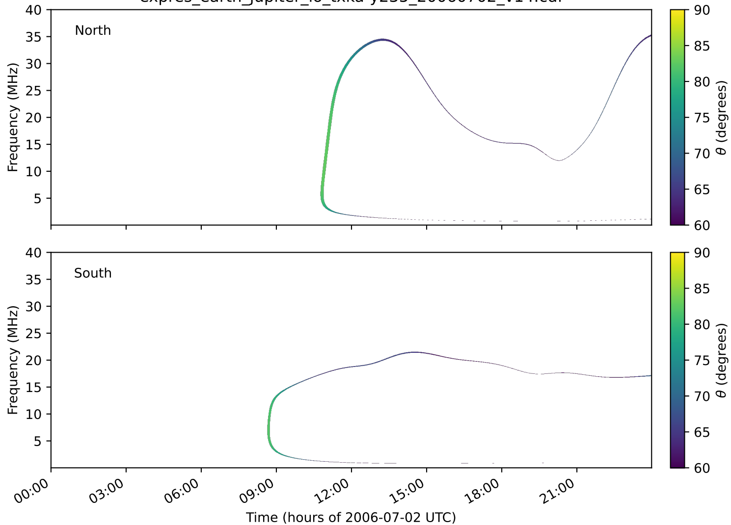
expres_earth_jupiter_io_txka-y235_20060702_v14.cdf
