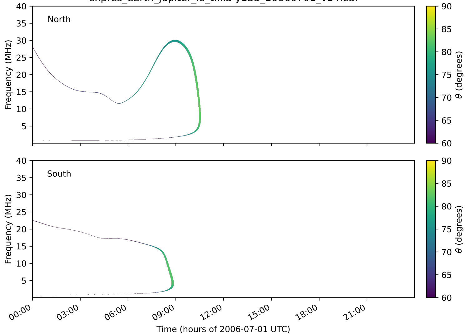
expres_earth_jupiter_io_txka-y235_20060701_v14.cdf
