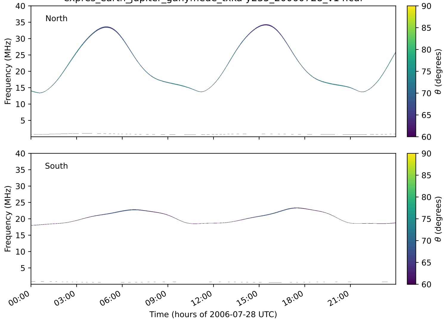
expres_earth_jupiter_ganymede_txka-y235_20060728_v14.cdf
