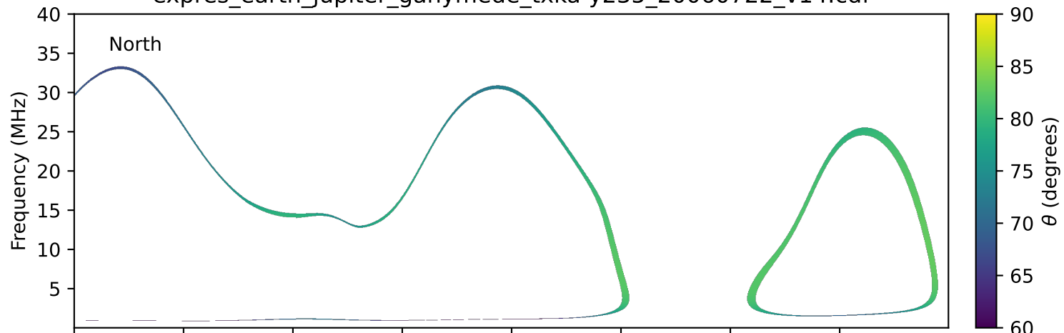
expres_earth_jupiter_ganymede_txka-y235_20060722_v14.cdf
