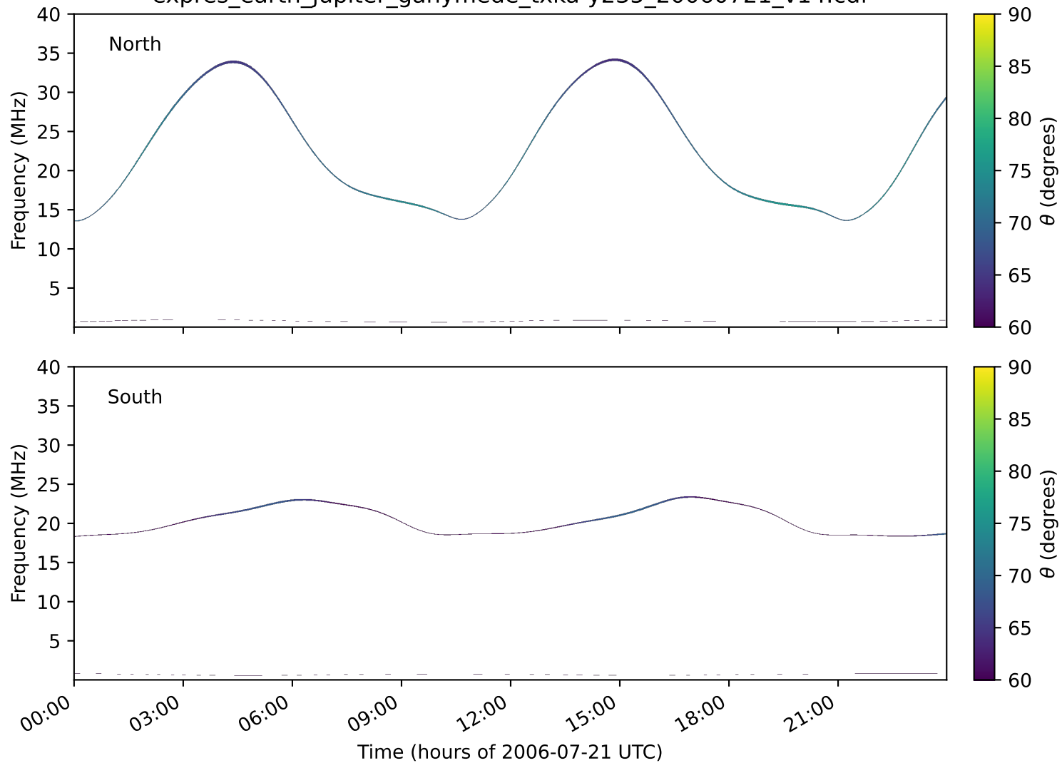
expres_earth_jupiter_ganymede_txka-y235_20060721_v14.cdf
