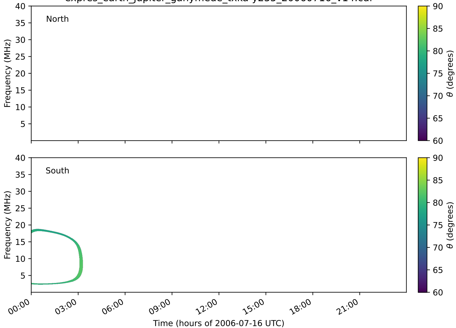
expres_earth_jupiter_ganymede_txka-y235_20060716_v14.cdf
