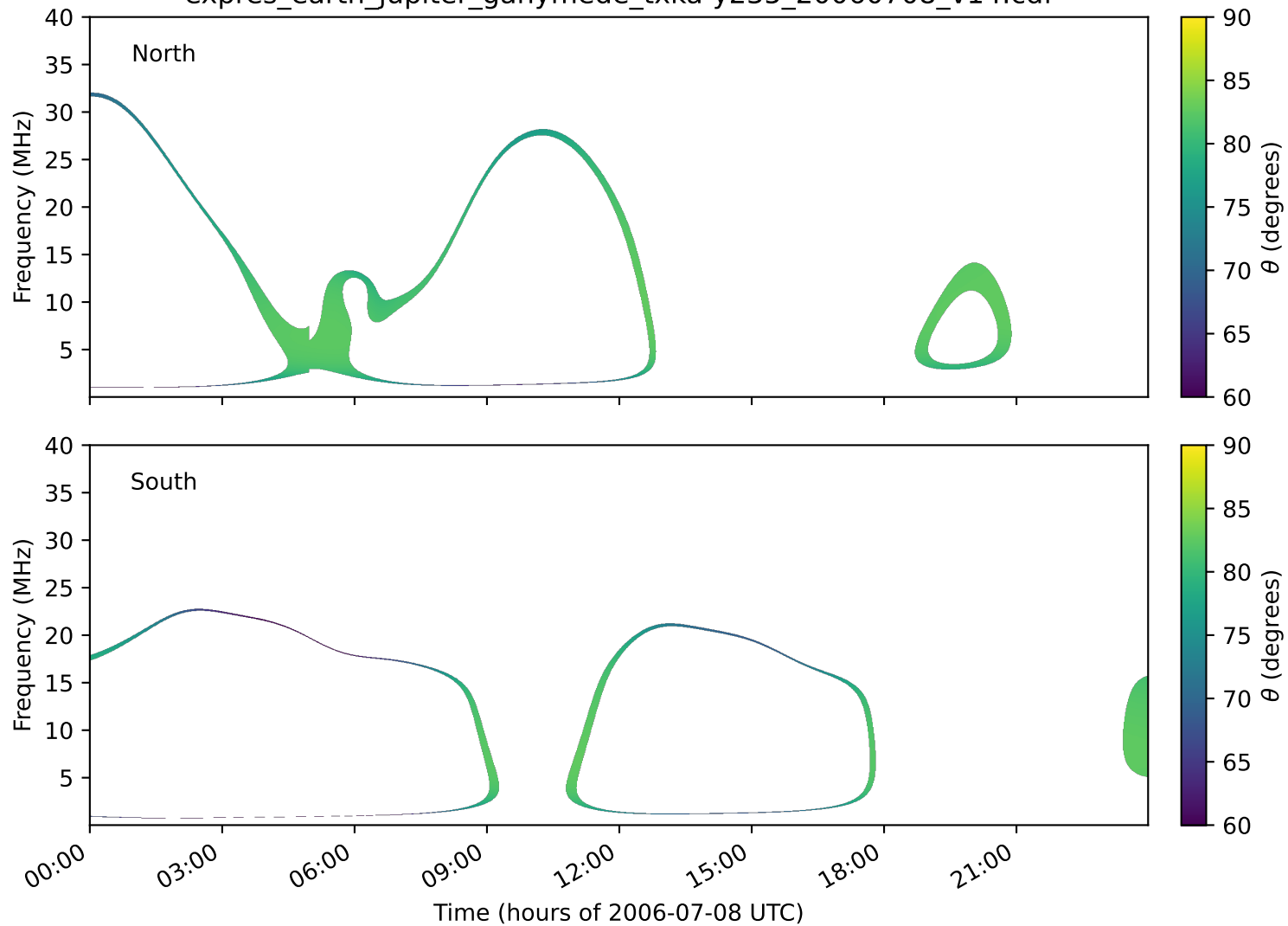
expres_earth_jupiter_ganymede_txka-y235_20060708_v14.cdf
