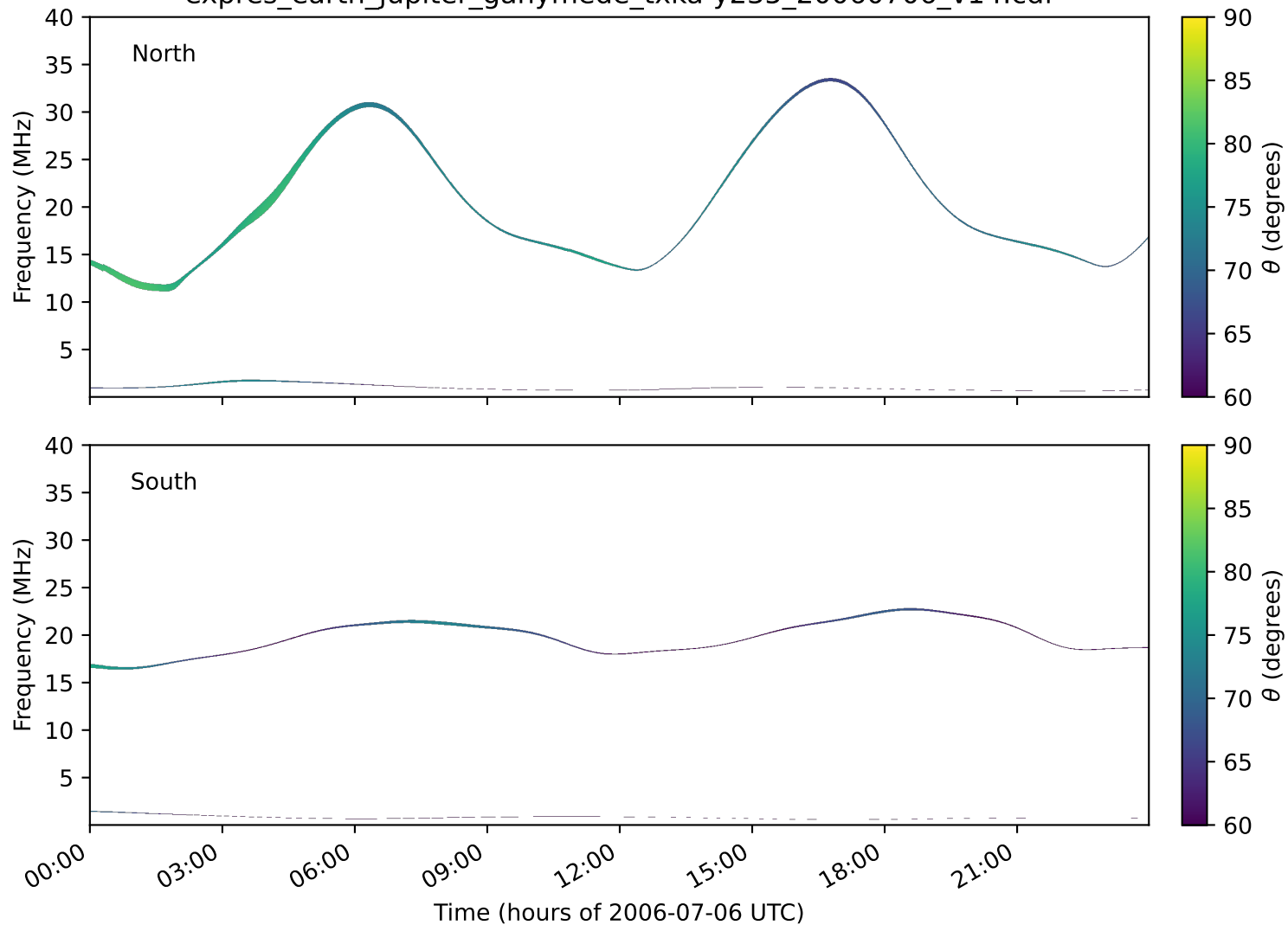
expres_earth_jupiter_ganymede_txka-y235_20060706_v14.cdf
