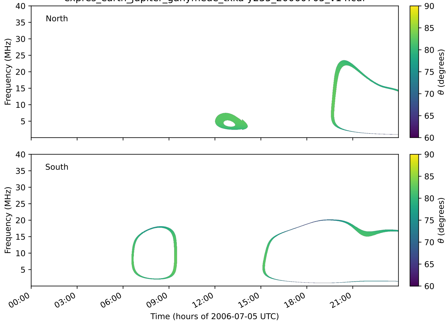
expres_earth_jupiter_ganymede_txka-y235_20060705_v14.cdf
