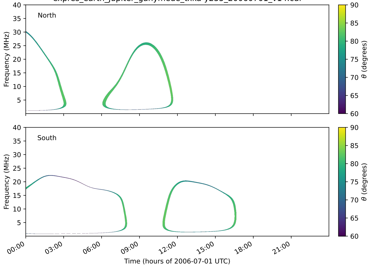
expres_earth_jupiter_ganymede_txka-y235_20060701_v14.cdf
