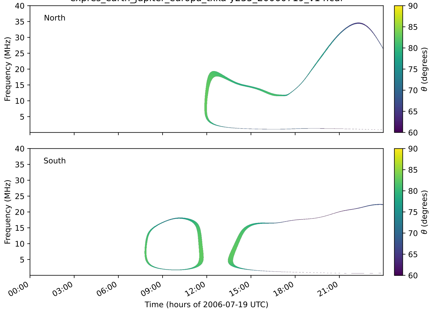
expres_earth_jupiter_europa_txka-y235_20060719_v14.cdf
