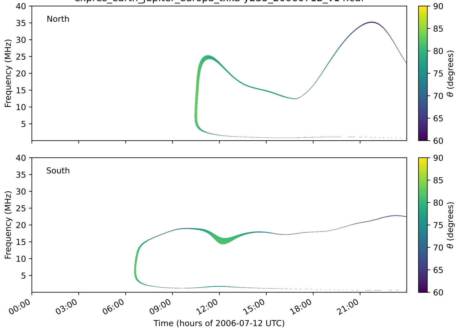
expres_earth_jupiter_europa_txka-y235_20060712_v14.cdf
