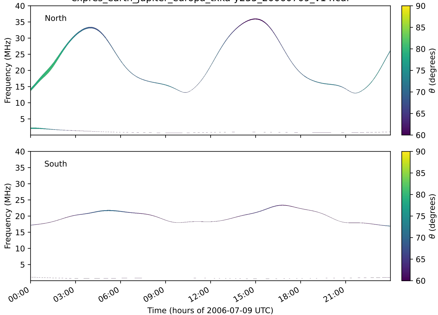
expres_earth_jupiter_europa_txka-y235_20060709_v14.cdf
