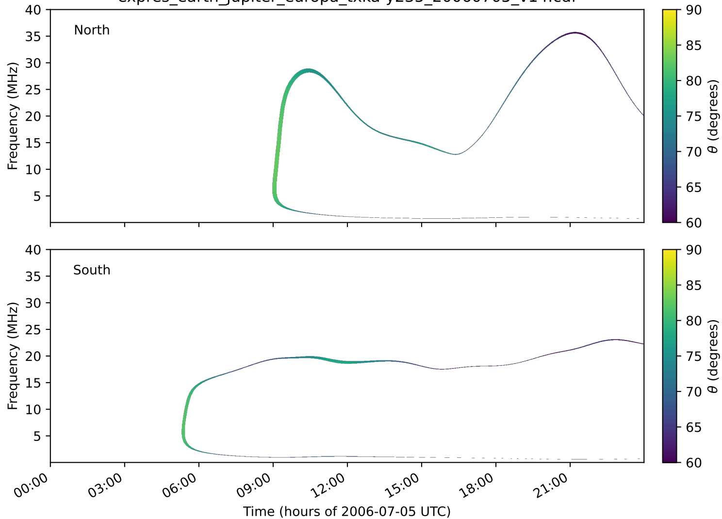
expres_earth_jupiter_europa_txka-y235_20060705_v14.cdf
