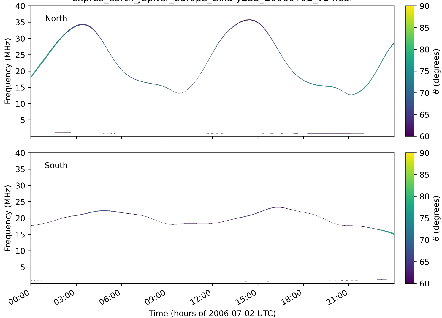
expres_earth_jupiter_europa_txka-y235_20060702_v14.cdf
