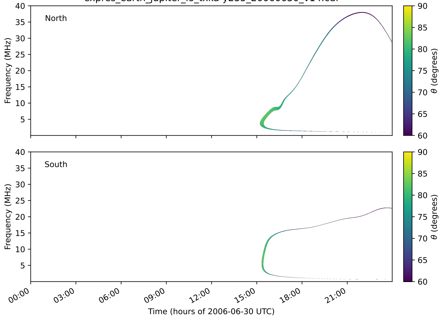
expres_earth_jupiter_io_txka-y235_20060630_v14.cdf
