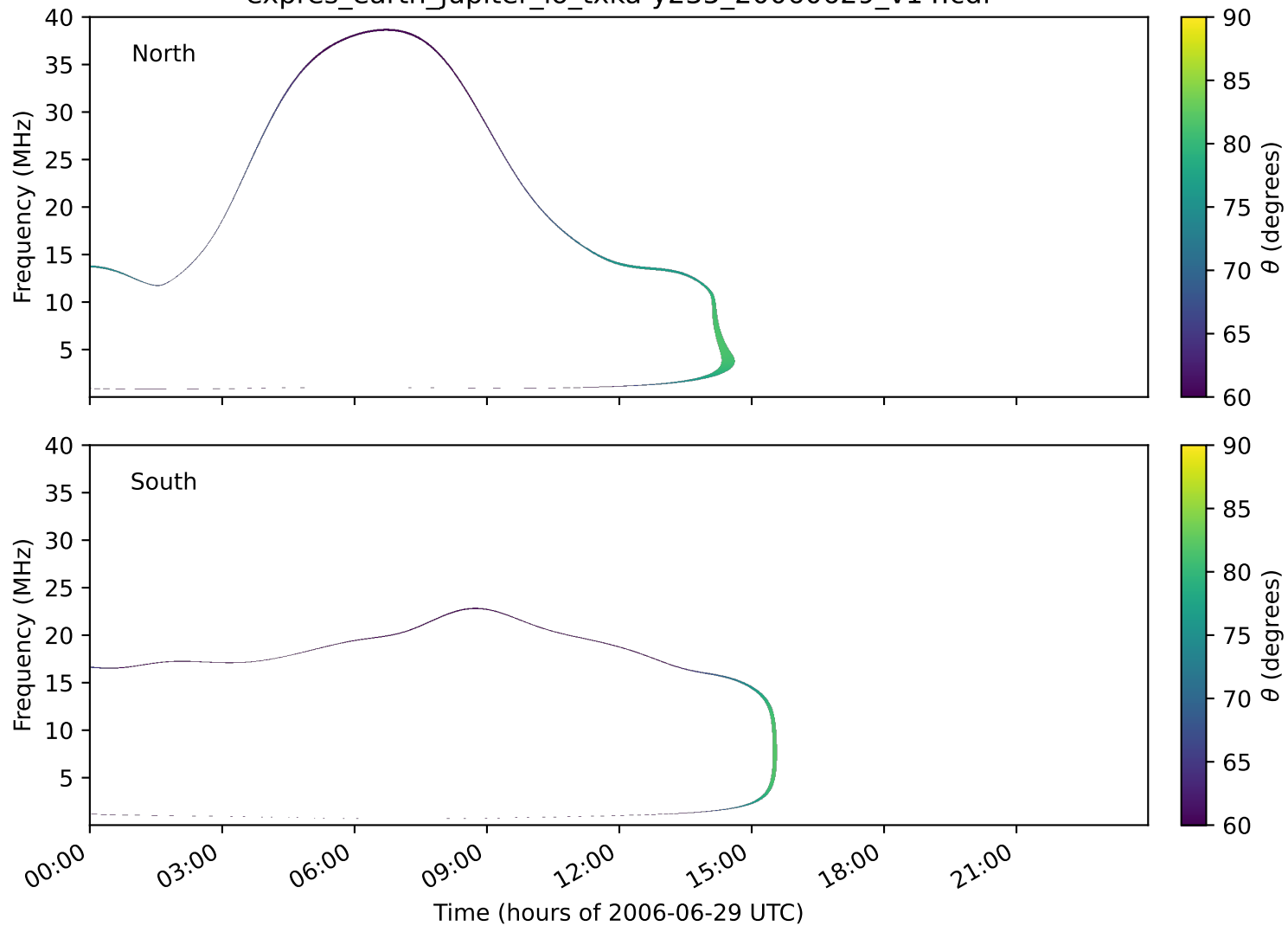
expres_earth_jupiter_io_txka-y235_20060629_v14.cdf
