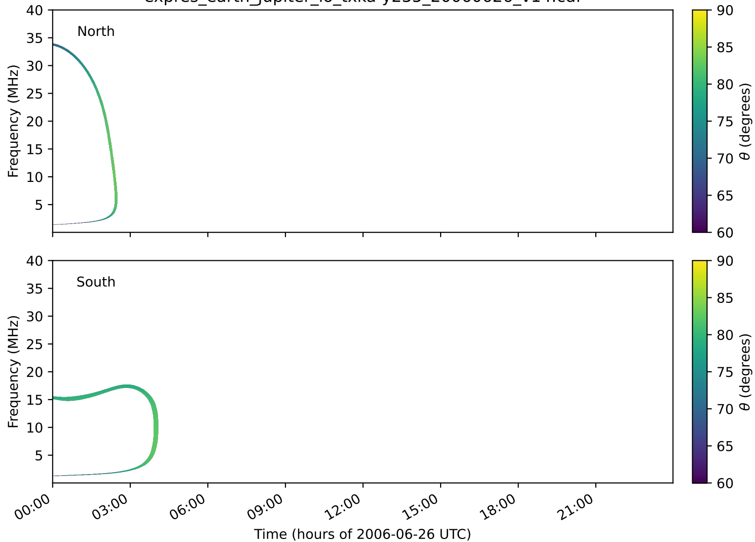
expres_earth_jupiter_io_txka-y235_20060626_v14.cdf
