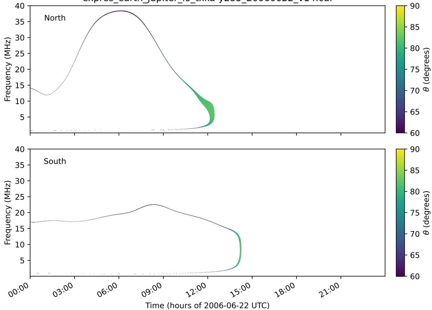
expres_earth_jupiter_io_txka-y235_20060622_v14.cdf
