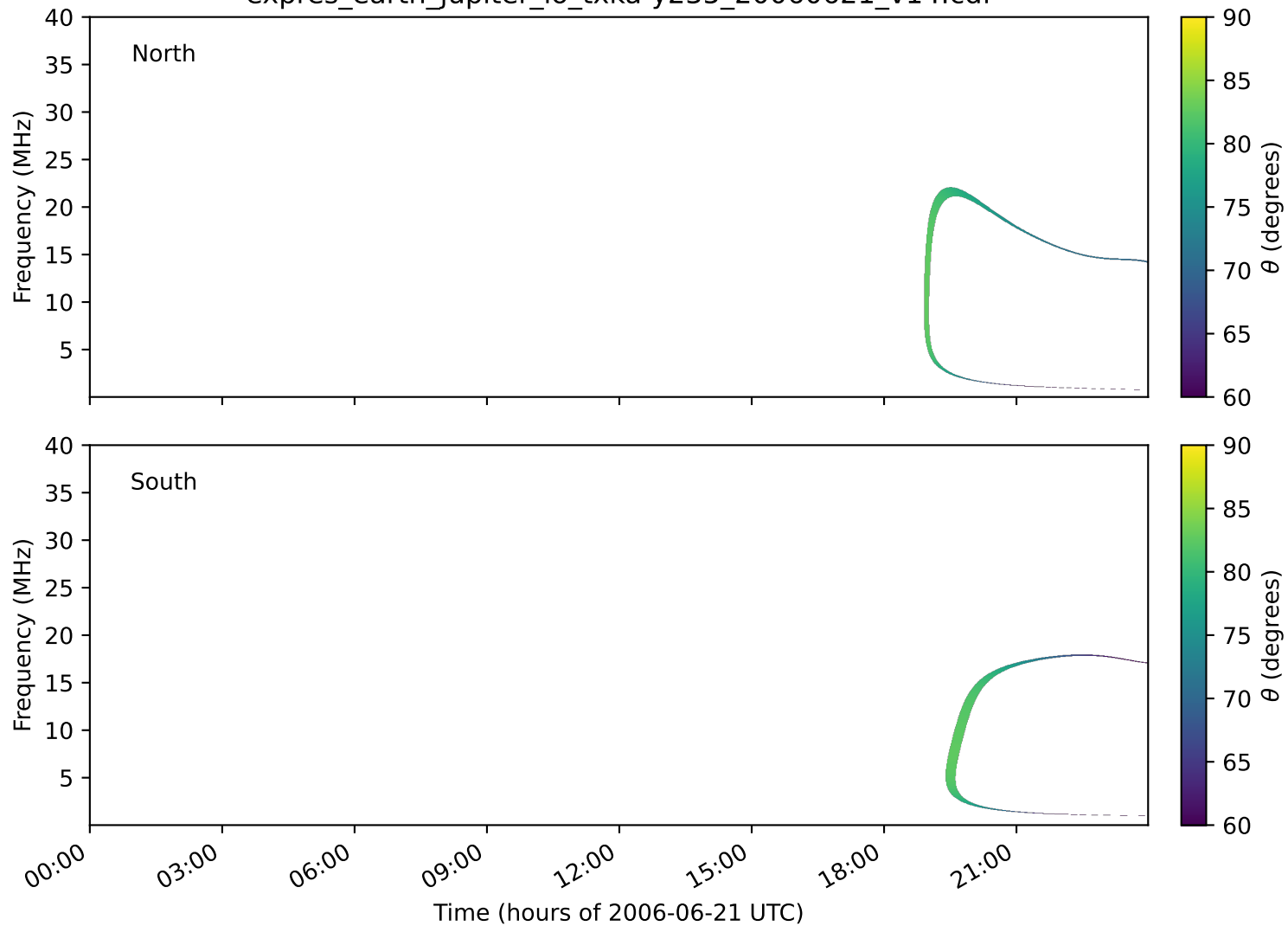
expres_earth_jupiter_io_txka-y235_20060621_v14.cdf
