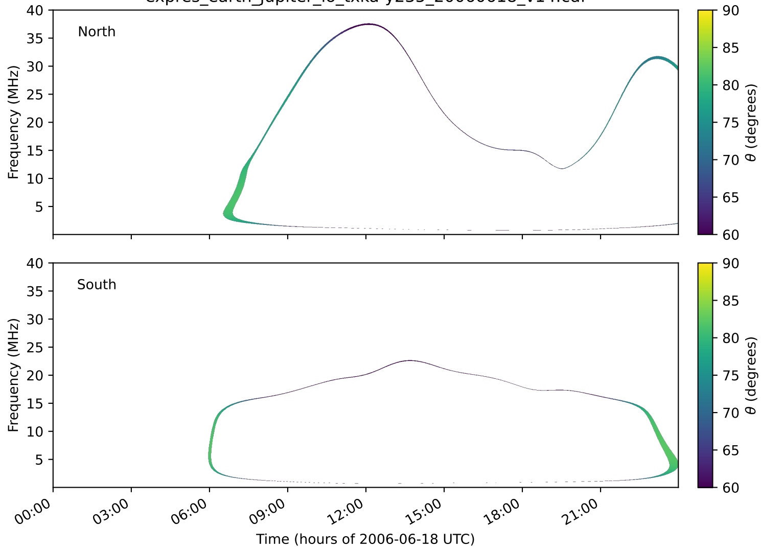
expres_earth_jupiter_io_txka-y235_20060618_v14.cdf
