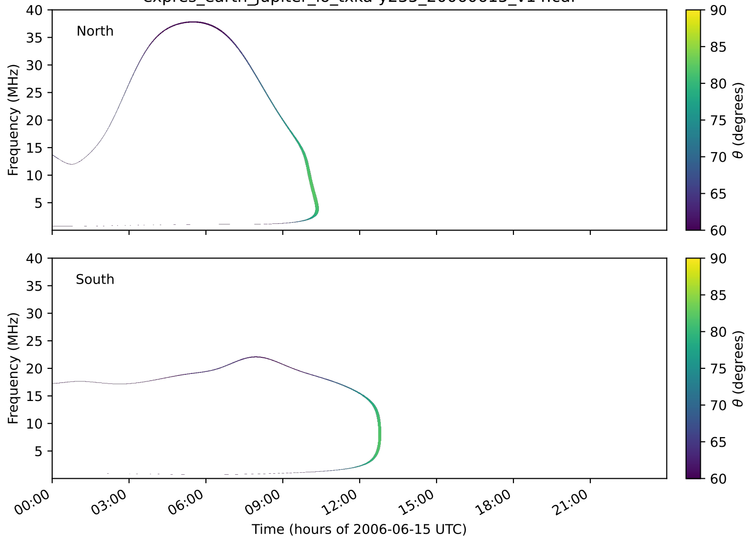
expres_earth_jupiter_io_txka-y235_20060615_v14.cdf
