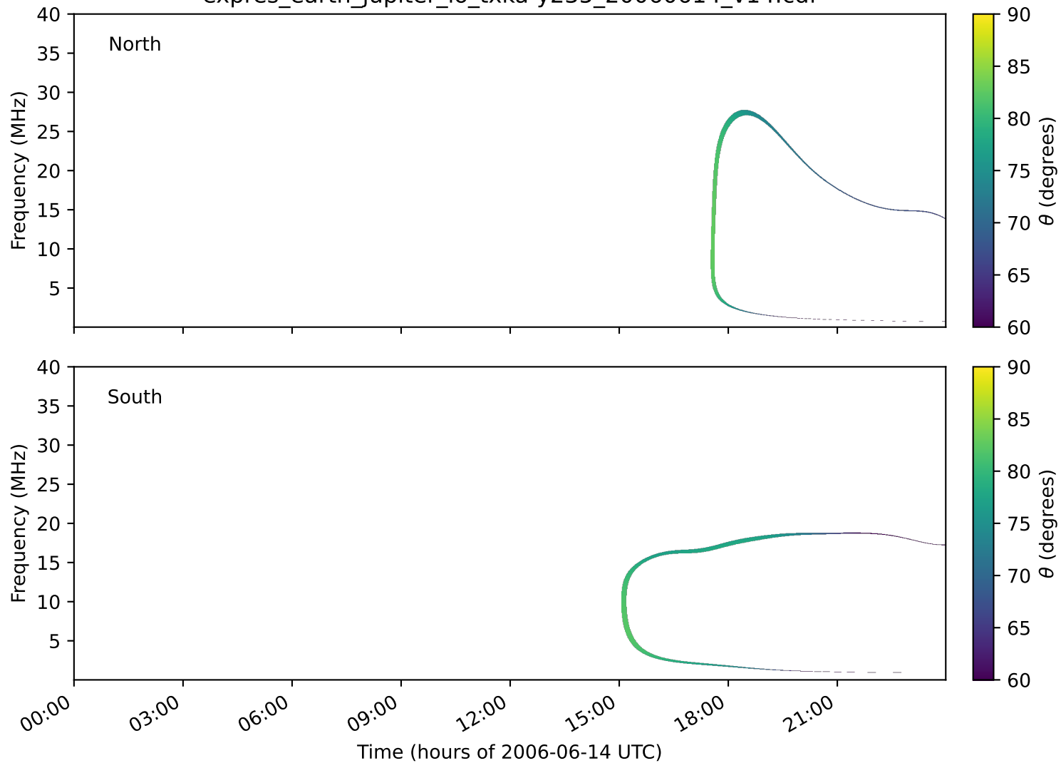
expres_earth_jupiter_io_txka-y235_20060614_v14.cdf
