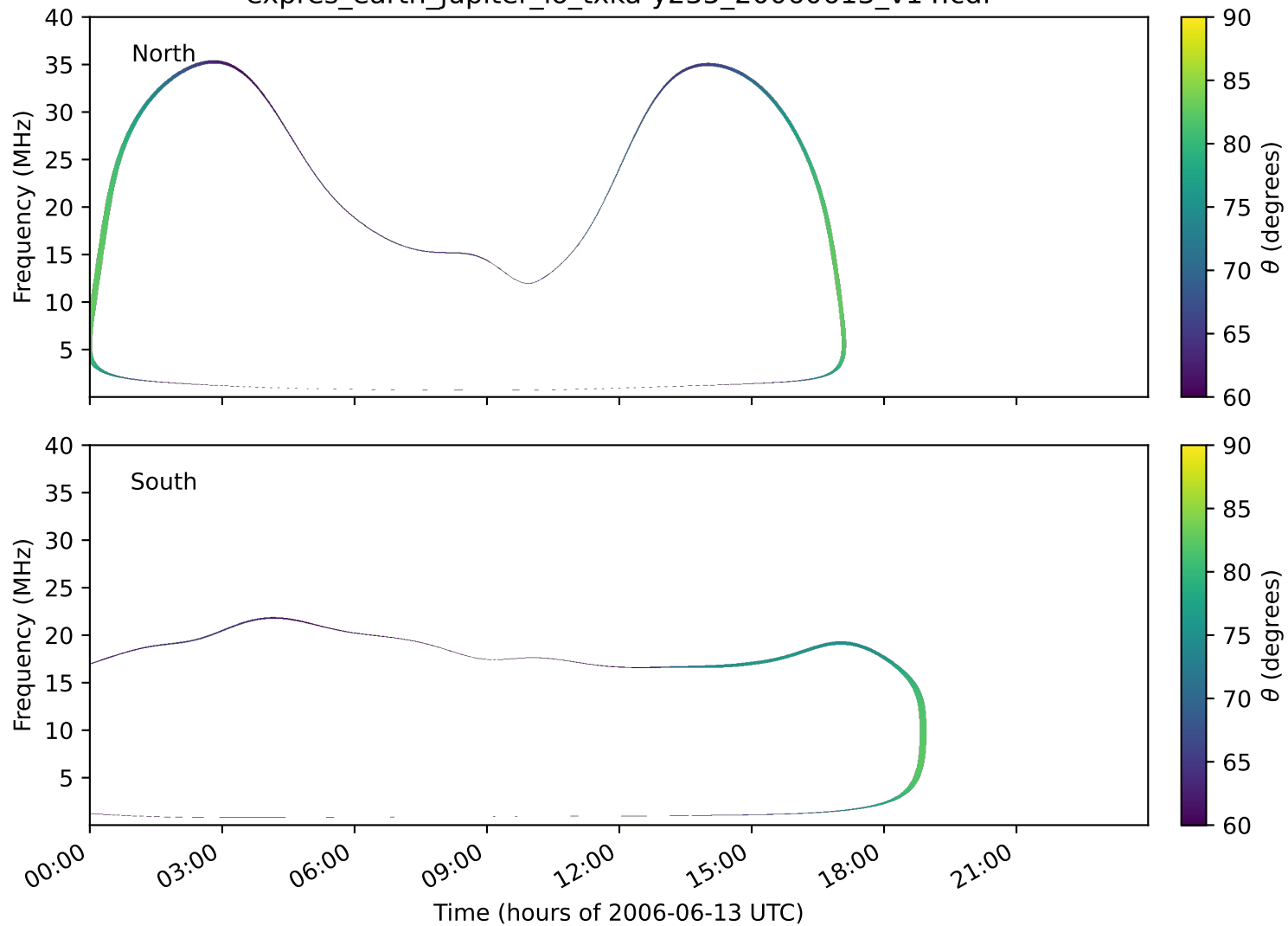
expres_earth_jupiter_io_txka-y235_20060613_v14.cdf
