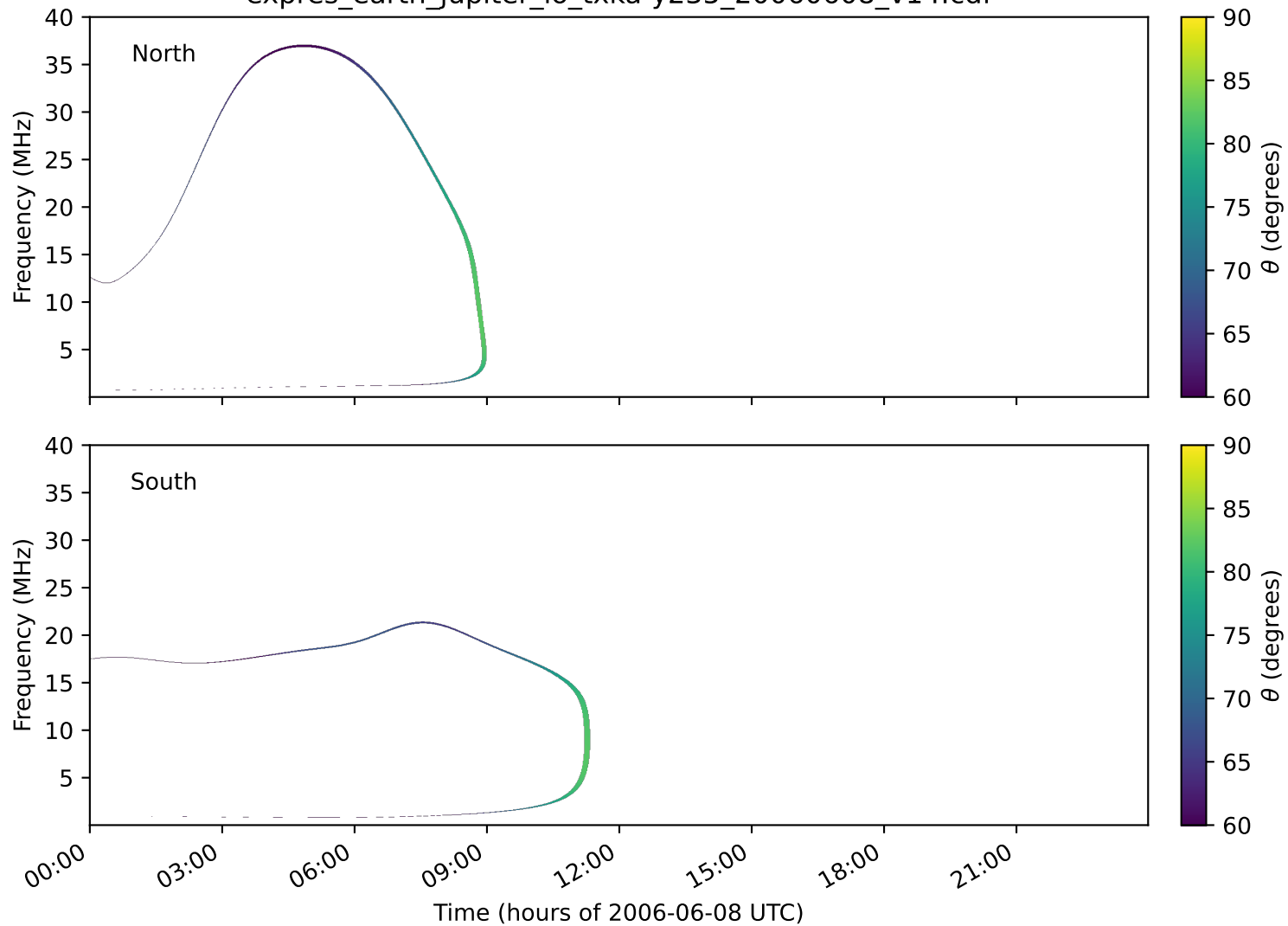
expres_earth_jupiter_io_txka-y235_20060608_v14.cdf
