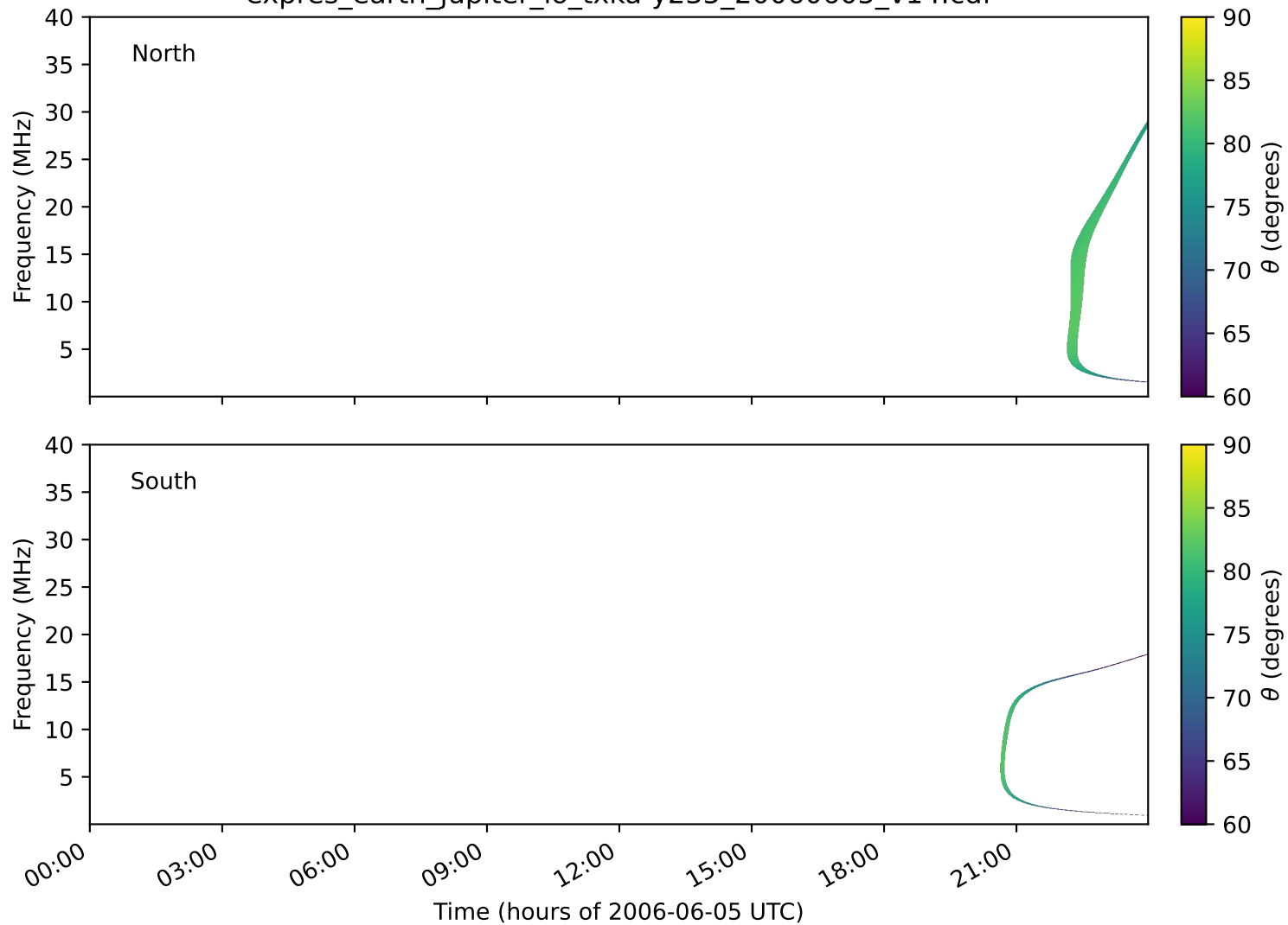
expres_earth_jupiter_io_txka-y235_20060605_v14.cdf
