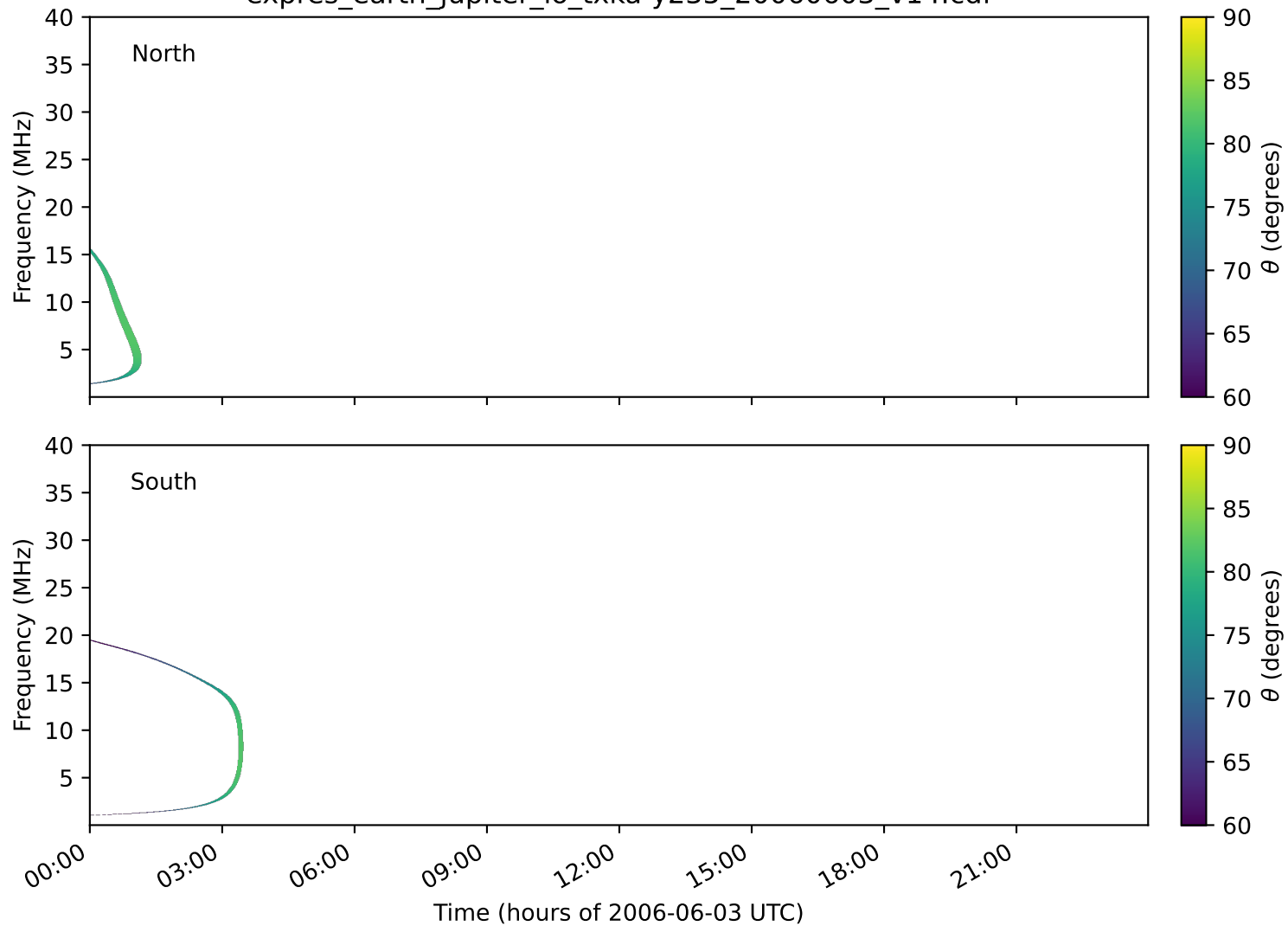
expres_earth_jupiter_io_txka-y235_20060603_v14.cdf
