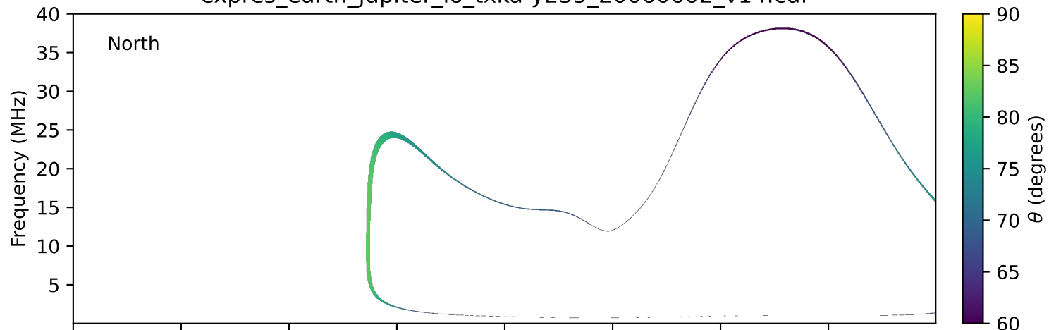
expres_earth_jupiter_io_txka-y235_20060602_v14.cdf
