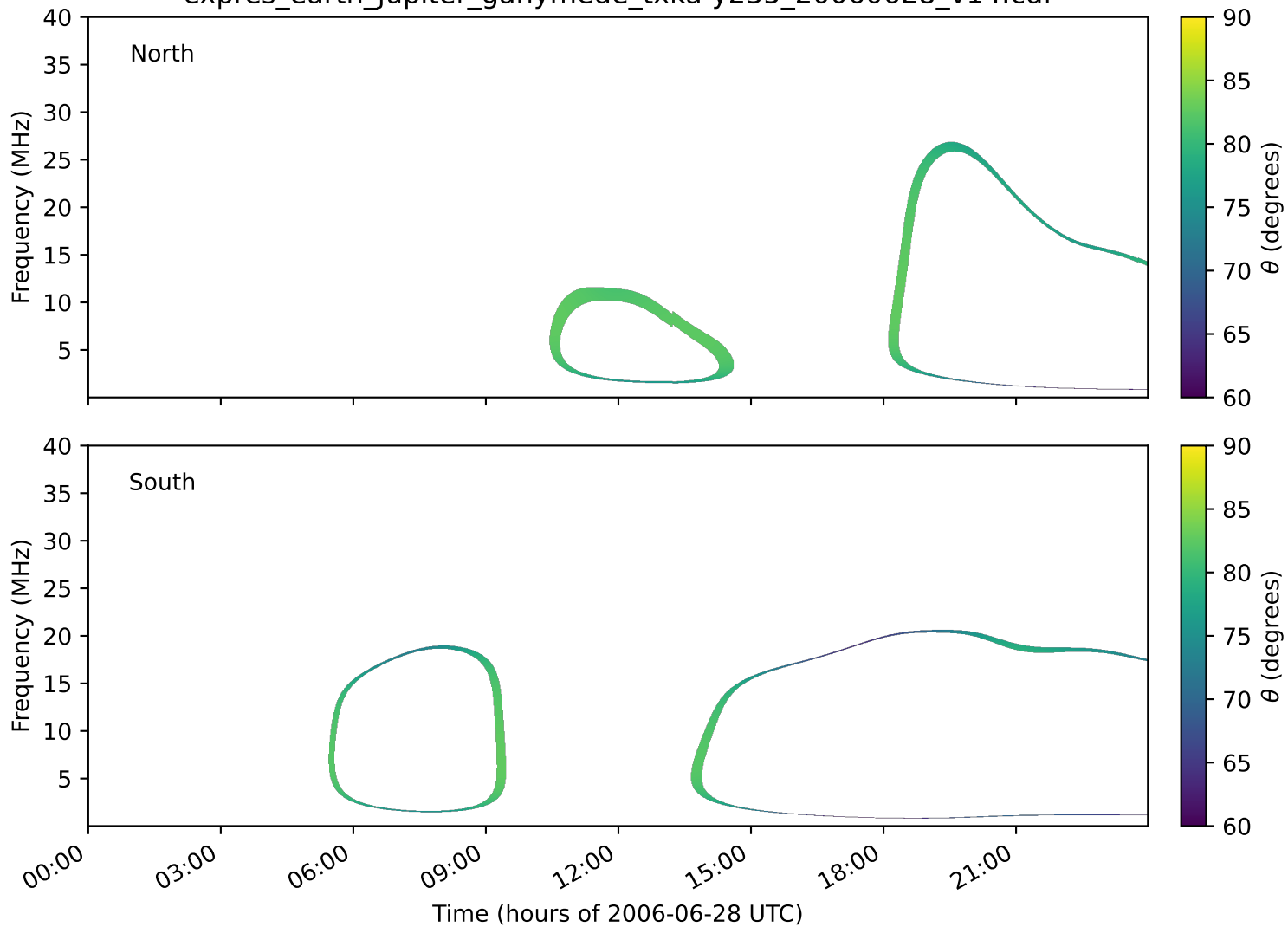
expres_earth_jupiter_ganymede_txka-y235_20060628_v14.cdf
