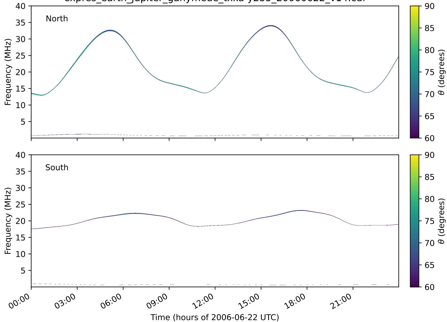
expres_earth_jupiter_ganymede_txka-y235_20060622_v14.cdf
