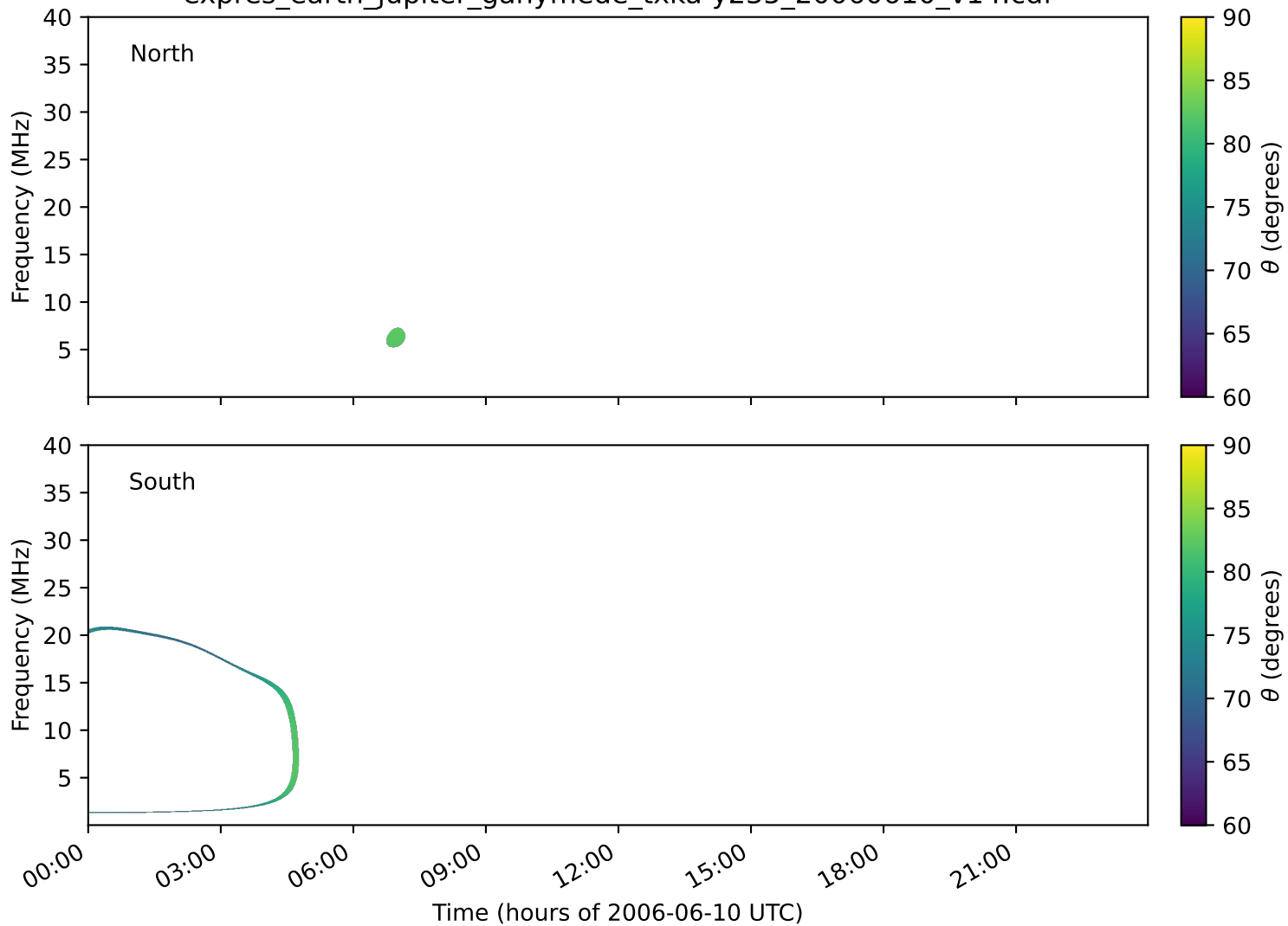
expres_earth_jupiter_ganymede_txka-y235_20060610_v14.cdf
