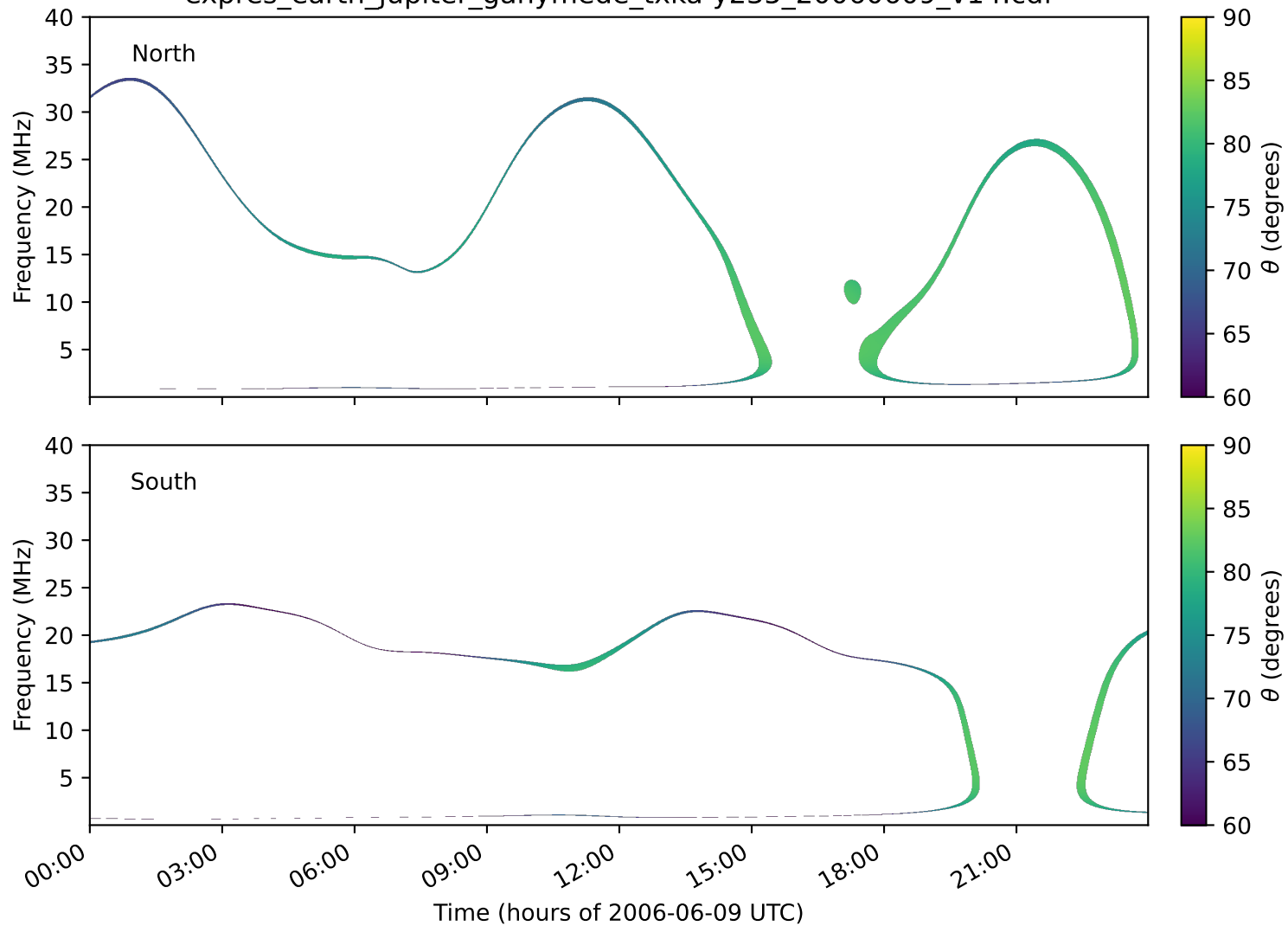
expres_earth_jupiter_ganymede_txka-y235_20060609_v14.cdf
