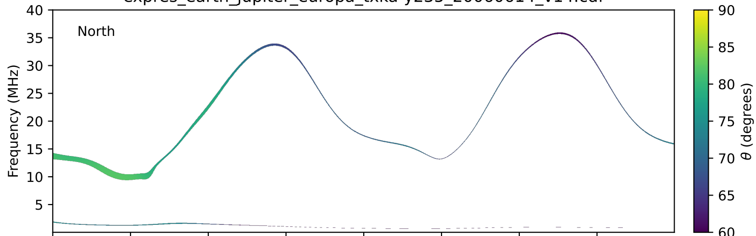
expres_earth_jupiter_europa_txka-y235_20060614_v14.cdf
